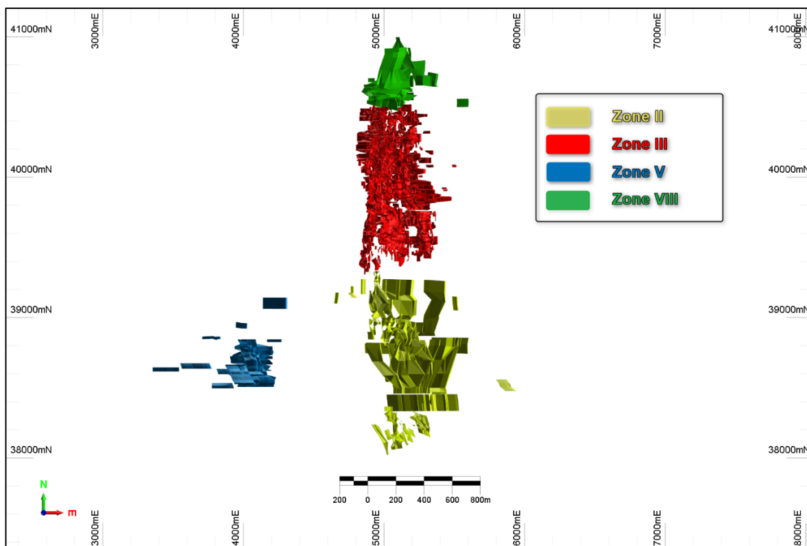
Figure 1: Plan showing mineralisation wireframes by zones.
